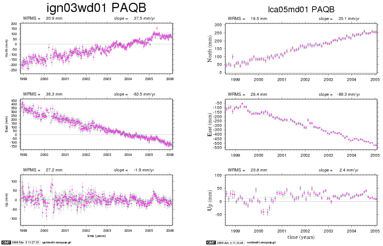
Figure 3: Station coordinate differences (STCD) for the PAQB station from the weekly IGN/JPL solution (available at ftp://cddis.gsfc.nasa.gov/pub/doris/products/STCD/ign03wd01/ign03wd01.STCD.paqb.gif ) and the monthly solution from LEGOS/CLS (available at ftp://cddis.gsfc.nasa.gov/pub/doris/products/STCD/lca05md01/lca05md01.STCD.paqb.gif ).
